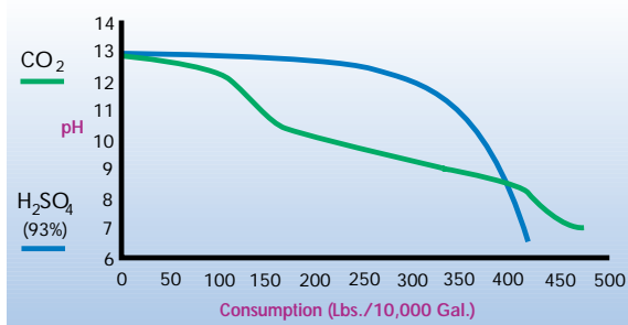
Typical Graph of CO 2 vs. H 2 SO 4 Effectiveness
